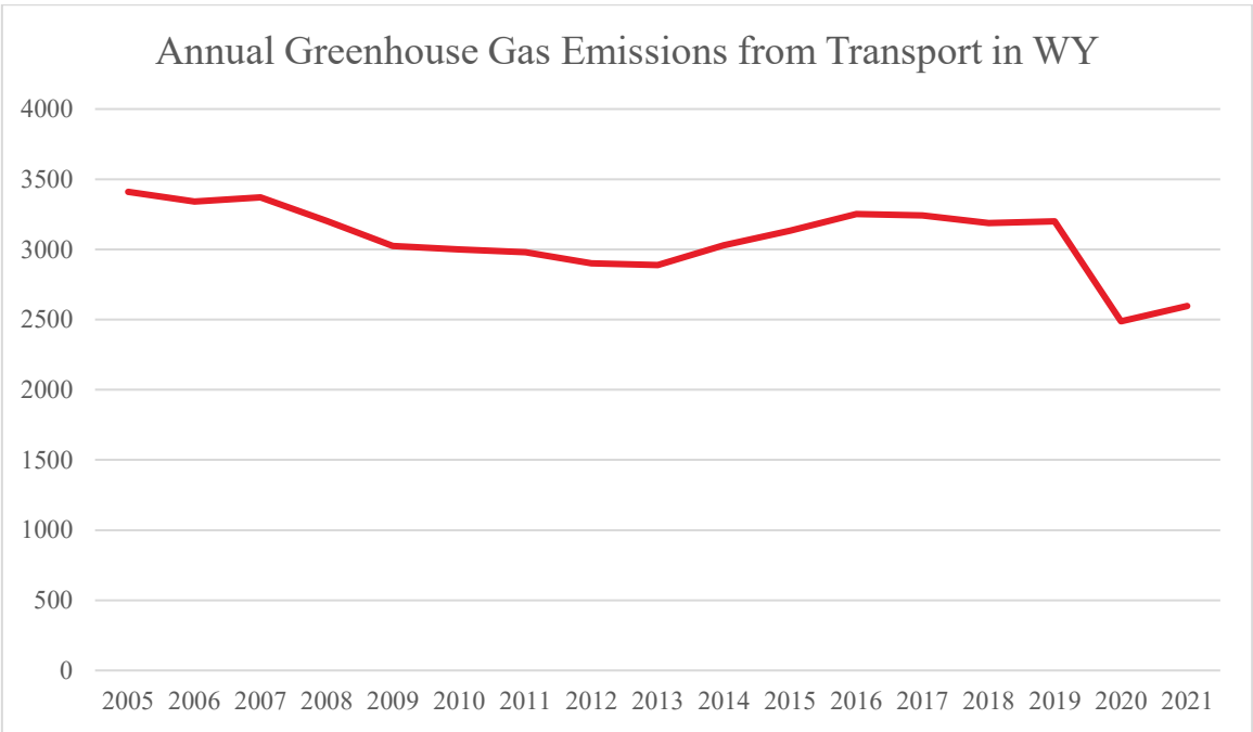
Figure 3: Annual Greenhouse Gas Emissions from Transport in West Yorkshire (2005 - 2021) Source: Department of Energy Security & Net Zero (2023a)
