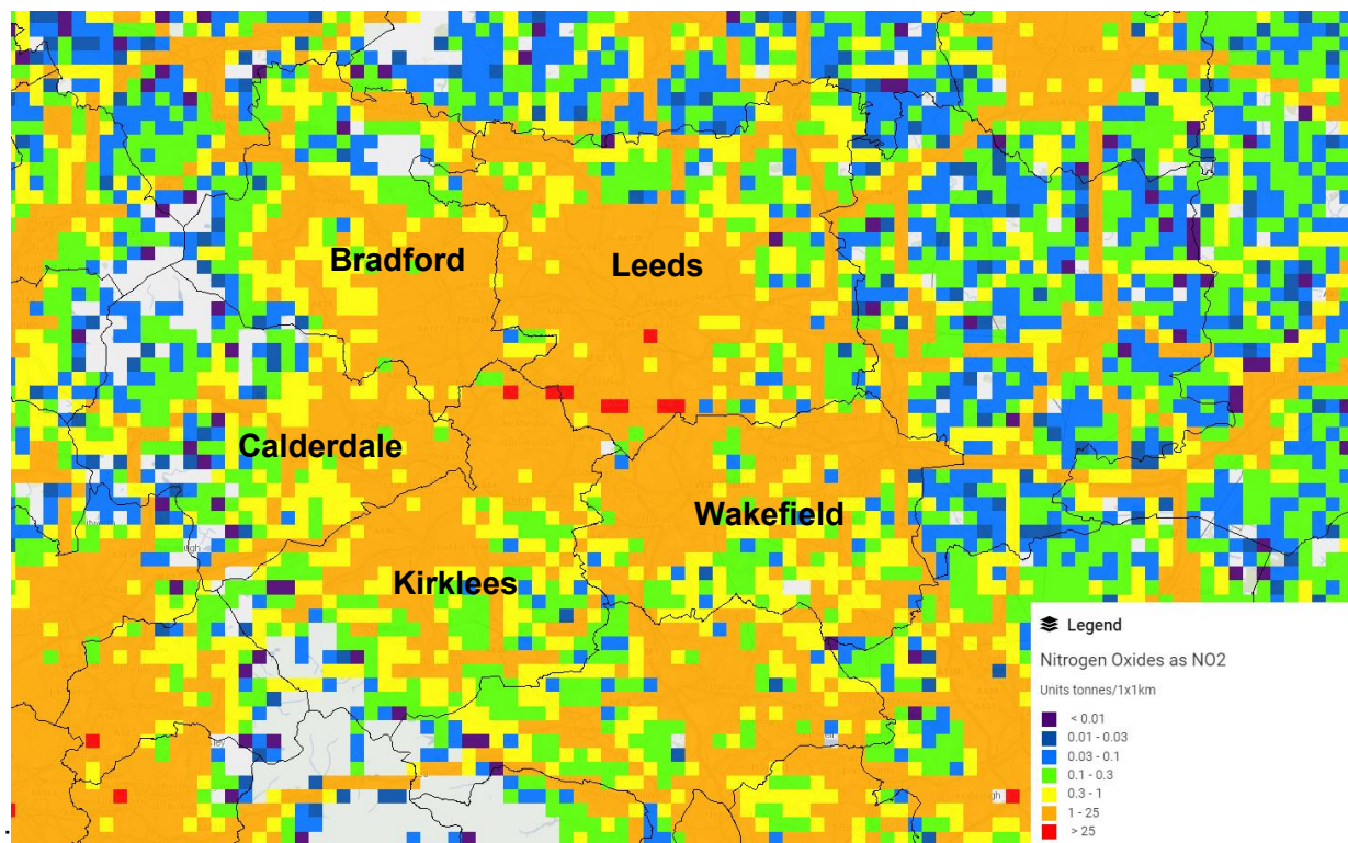
Figure 5: O2 Emissions from Road Transport in West Yorkshire Source: National Atmospheric Emissions Inventory (2021)
